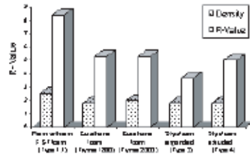
FOAM INSULATION COMPARISON USING 1 in. Thickness
